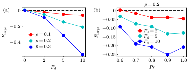
Fig. 6. The active diffusiophoretic force on the frozen passive colloidal particle as a function of (a) the self-propelling force F_d with Pr = 1.0 and (b) the transition probability Pr for different F_d . Here, the positive direction of the force points to the sink of the ABPs (the system center).
