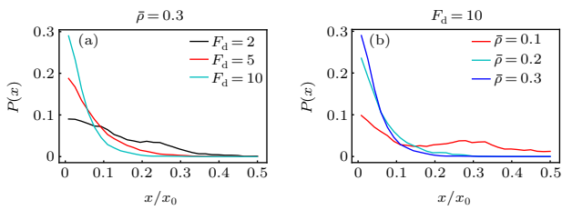
Fig. 5. Probability distribution of the active diffusiophoretic passive colloidal particle (a) for different self-propelling force F_d and (b) for different mean packing fractions of the solvent particles \bar{\rho} , with Pr = 1.0 being fixed.
